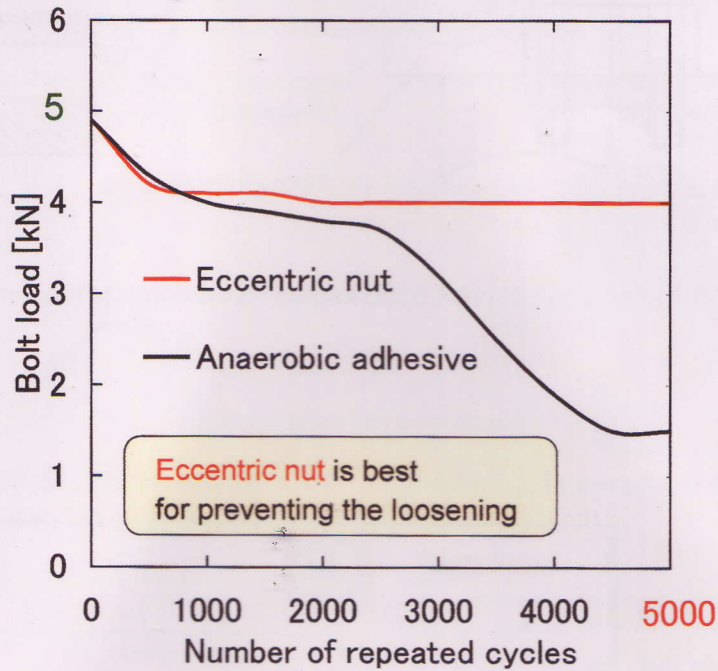
Figure-4 (a) The result in the loosening test using Junker's machine (Bolt preload is 5kN, the maximum number of repeated cycles is 5000)
